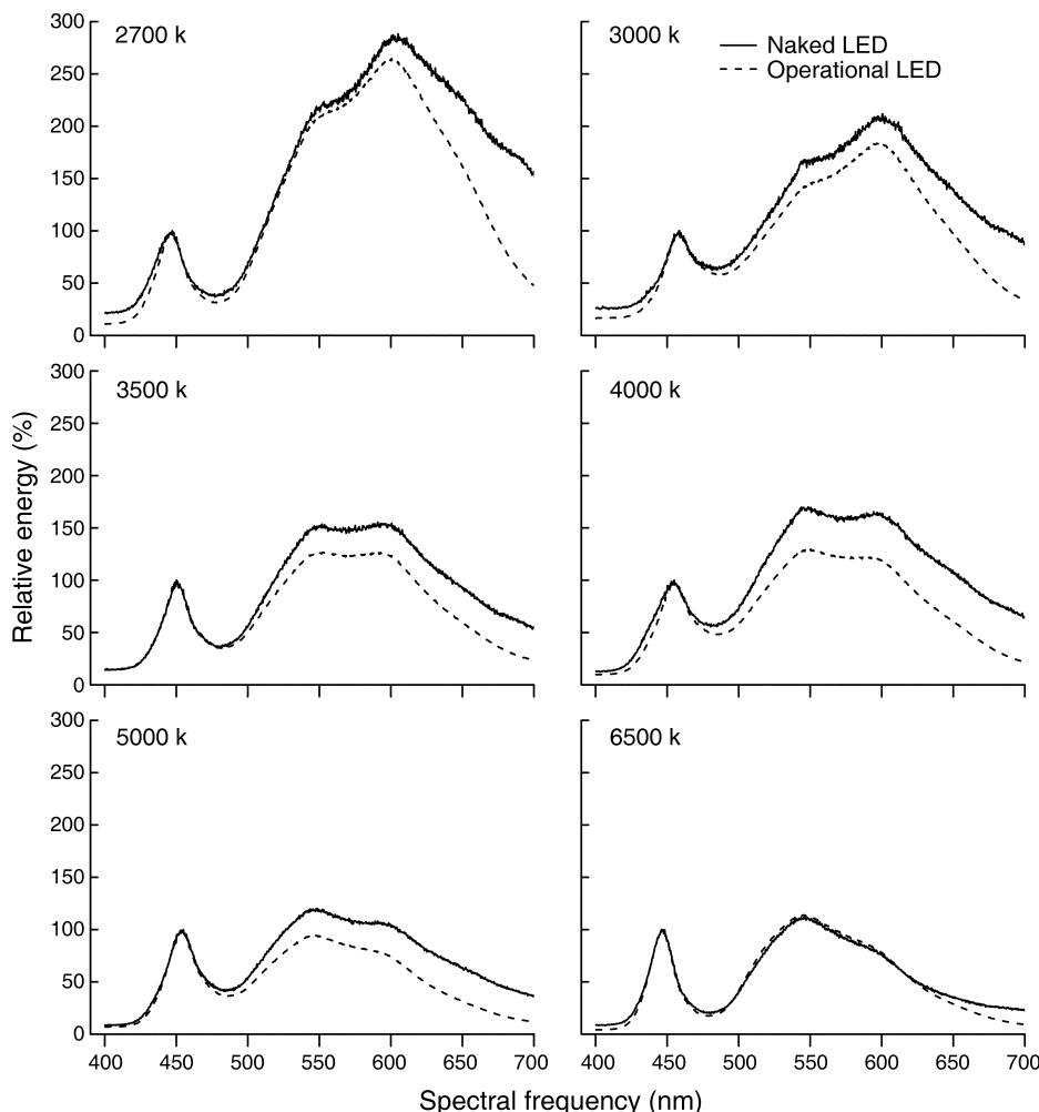
FIG. 2. Relative spectral emission of “white” LED of differing color temperatures. Emission spectra were measured using an OceanOptics USB2000 fiber-coupled spectrometer (Ocean Optics, Dunedin, Florida, USA) with an integration time of 100 ms. Emission spectra are normalized to the maximum spectral intensity in the 400–500 nm range, as insects are most attracted to this portion of the visible spectrum. The shape and form of the curve in the blue-green region is almost identical between naked LEDs and operational LEDs where measurements were taken behind the Perspex and Tanglefoot-coated Mylar.
