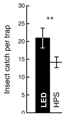
FIG. 3. Number of flying invertebrates (standardized by the 3.7–4.2 h trapping duration) caught in light traps equipped with LED or HPS light. Values are means \pm SE, n = 5 replicates. ** P < 0.01 .
