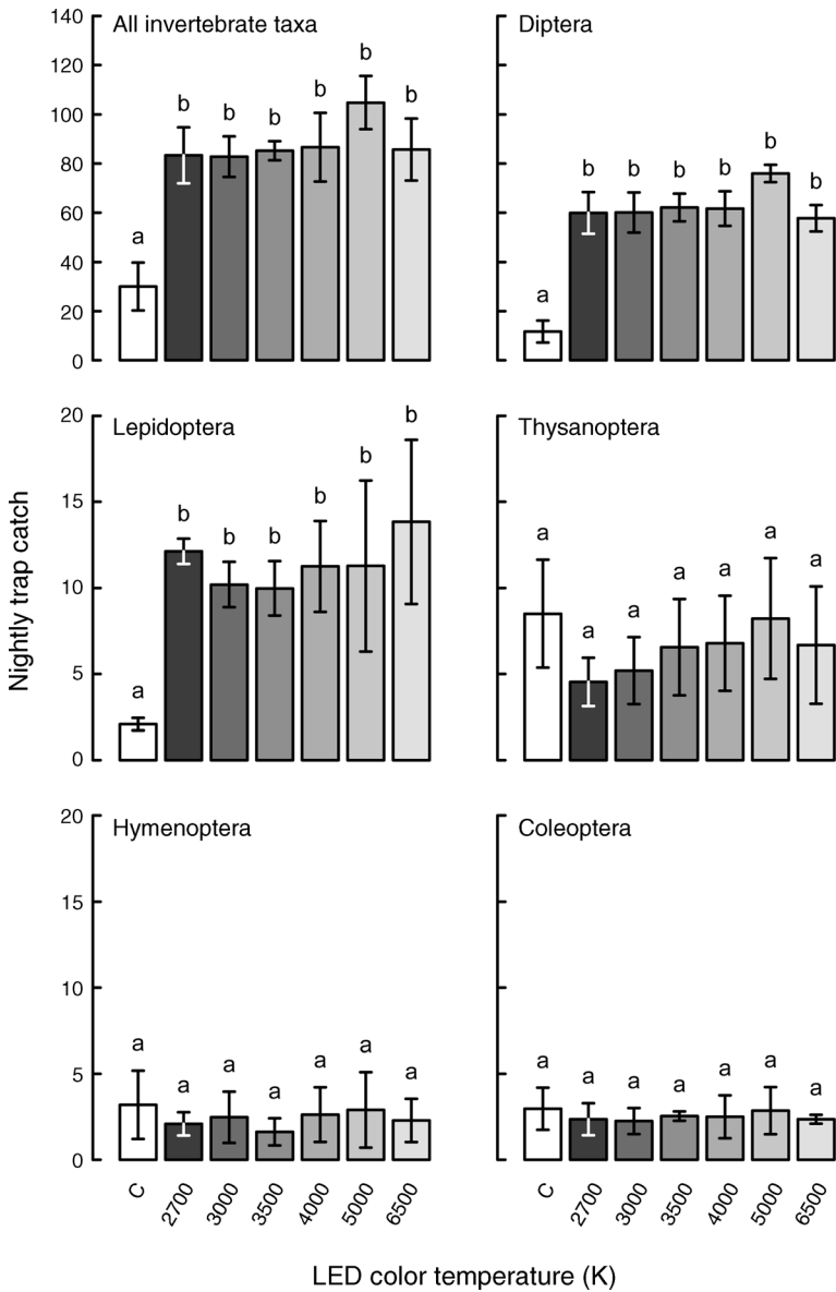
FIG. 4. Effect of LED color temperature on flying invertebrates trap catch over a 4-h sampling period; C is the control trap, values below the bars indicate the color temperature in Kelvin ( n = 3 blocks, values are means \pm SE). Different lower case letters indicate statistically significant differences at \alpha = 0.05 (multiple comparison procedure using Tukey contrasts).
