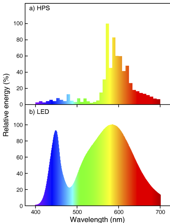
FIG. 1. Relative spectral emission of (a) high-pressure sodium (HPS) lamp (Sunlux ACE, NH-360 FLX; EYE Lighting, Wacol, Queensland, Australia) and (b) light-emitting diode (LED) 4000 K color temperature high bay lamp (LUXEON M, LXR7-SW40; Koninklijke Philips, Amsterdam, The Netherlands). Emission spectra are normalized to the spectrum with the maximum intensity and were kindly provided by each manufacturer.
